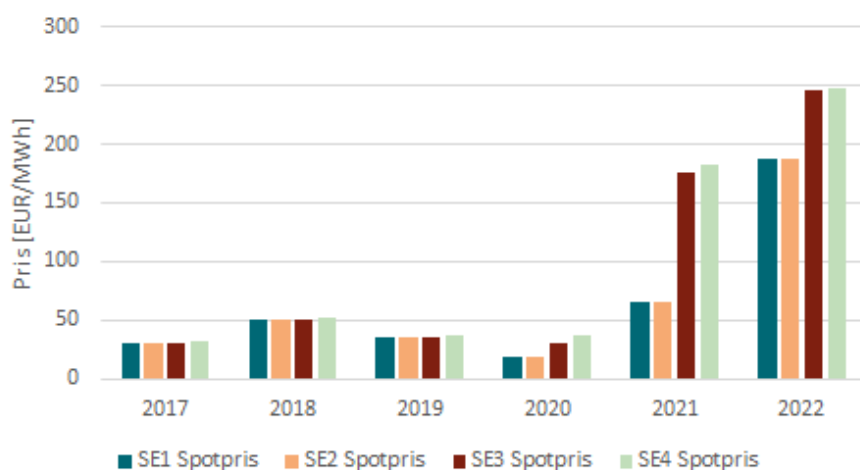
Figur 12 Elpriser (spotpriser) i december
