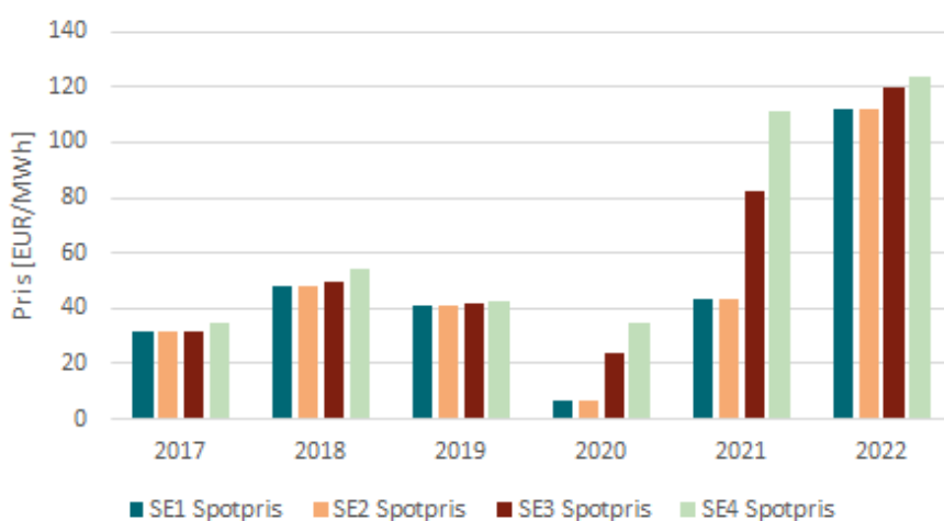
Figur 13 Elpriser (spotpriser) i november
