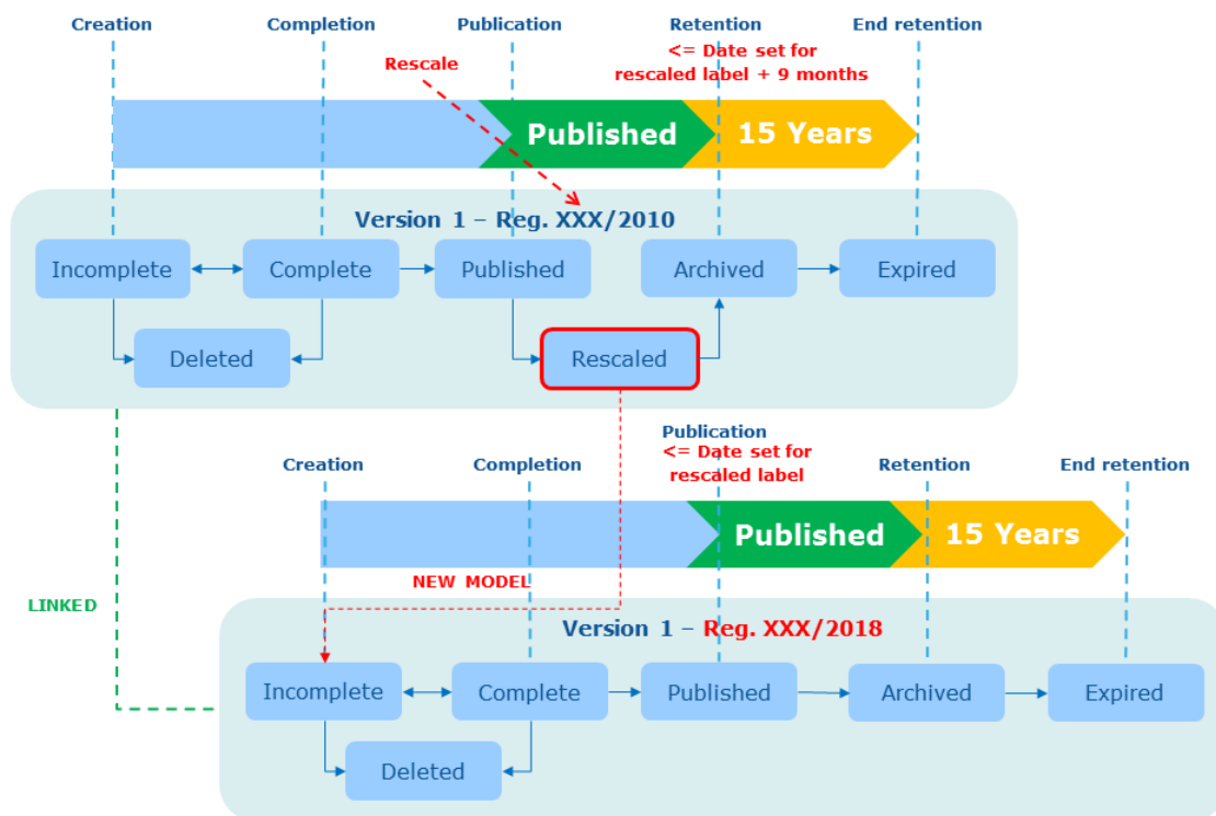
Figure 7 Model rescaling
