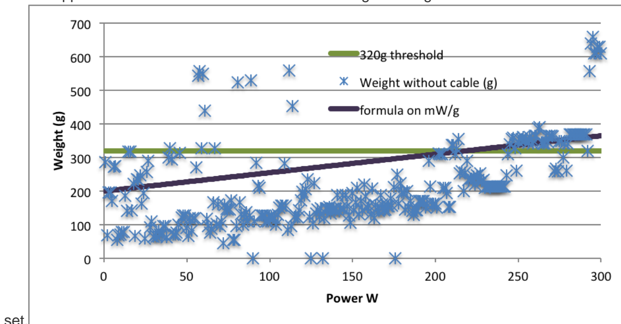
Figure 5 - Potential weight requirements against EPS data set.
