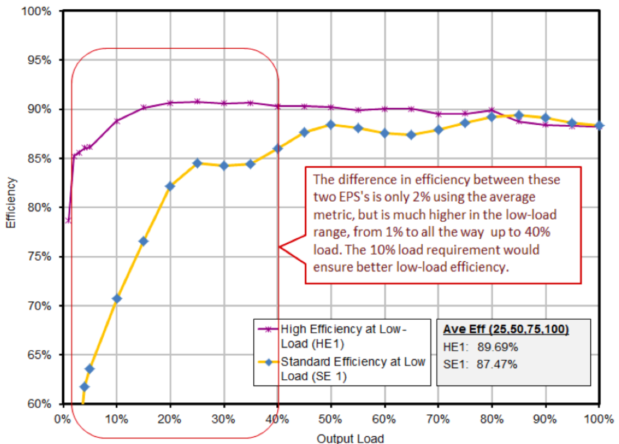
Figure 2 – Low load efficiency variation for two EPS at 230V. 13
