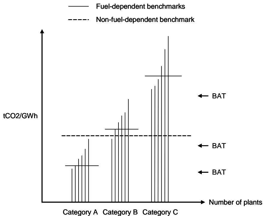
Figure 2. Examples of benchmarks (horizontal lines) with and without links to the fuels used, together with carbon dioxide intensities (vertical lines) for plants in different fuel categories.
