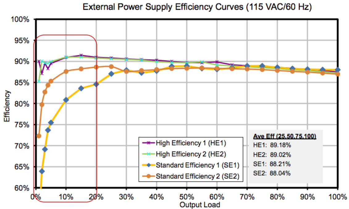
Figure 1 – Large differences in low-load EPS efficiency 23
