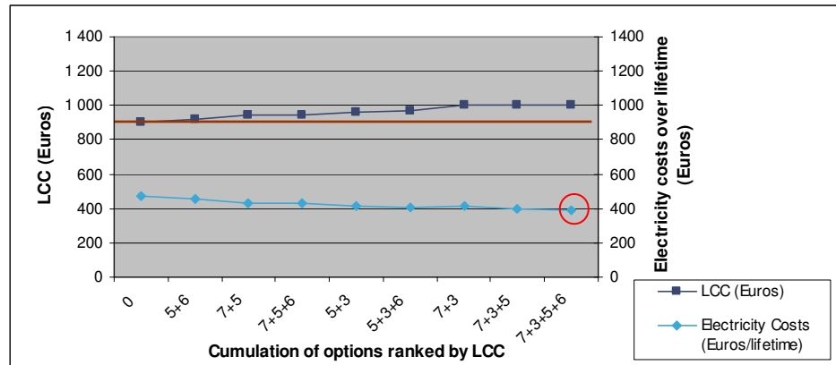
Figure 183: LCC Curve; environmental performance expressed in total electricity costs for the vented base case cumulating options
